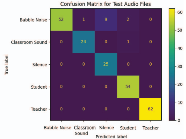
Fig.2. Confusion matrix of the testing data
