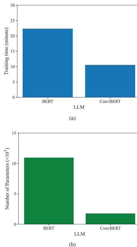
Fig. 3. Comparison between BERT and ConvBERT. (a) Training time comparison; (b) Number of parameters comparison.
